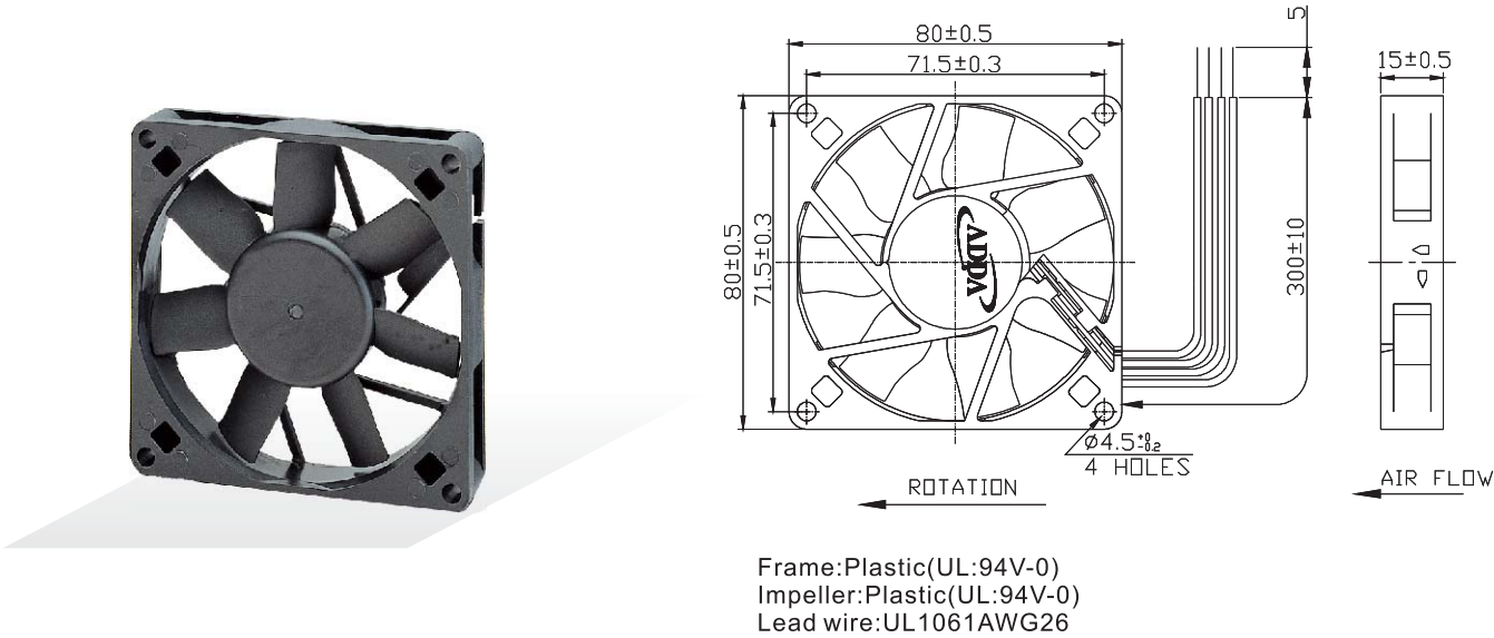
External Dimensions
